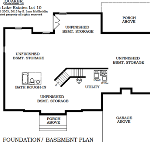
FOUNDATION/ BASEMENT PLAN
