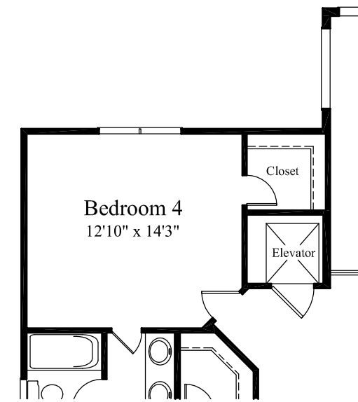
Partial Second Floor Plan w/ Opt. Elevator
