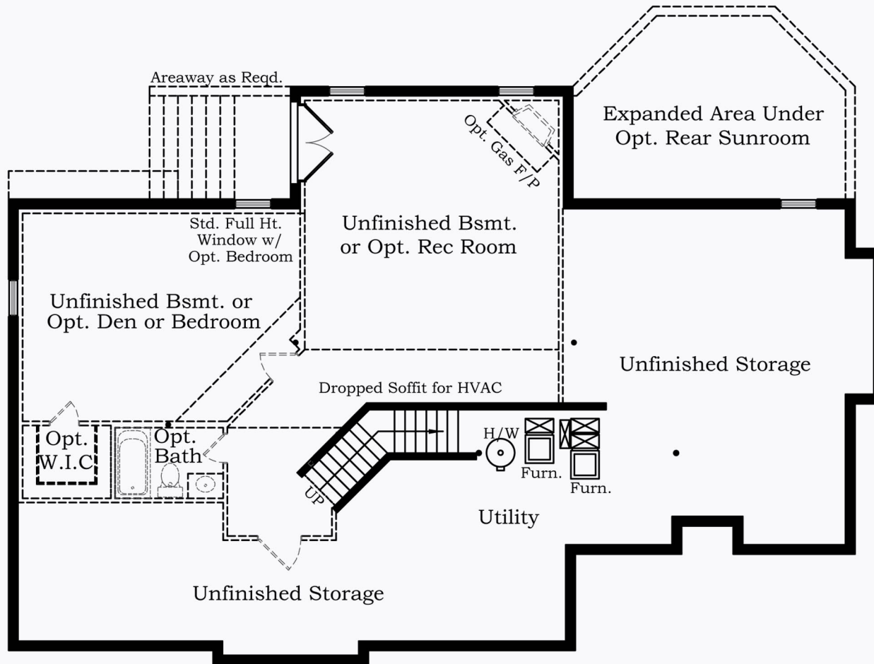
Lower Level
