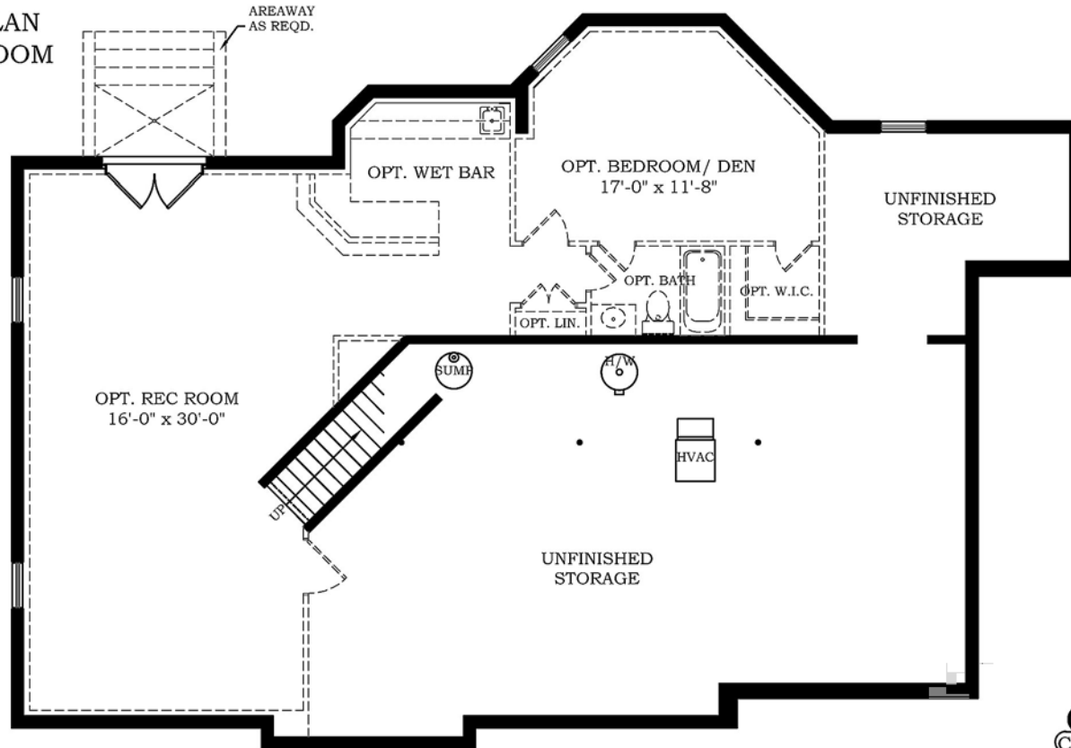
PARTIAL LOWER LEVEL PLAN W/ OPT. MAIN LEVEL BR ADDITION
