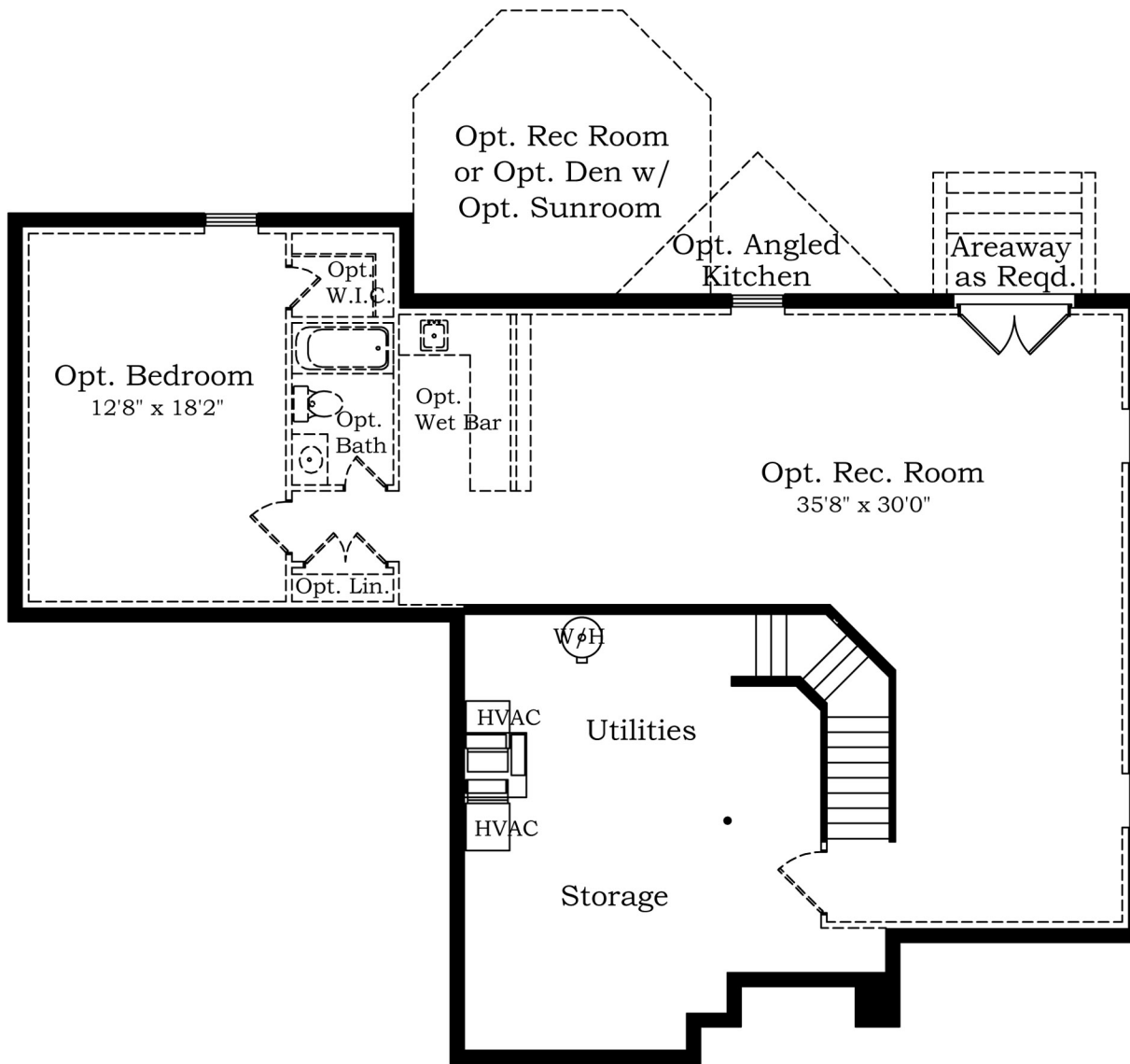
Lower Level
