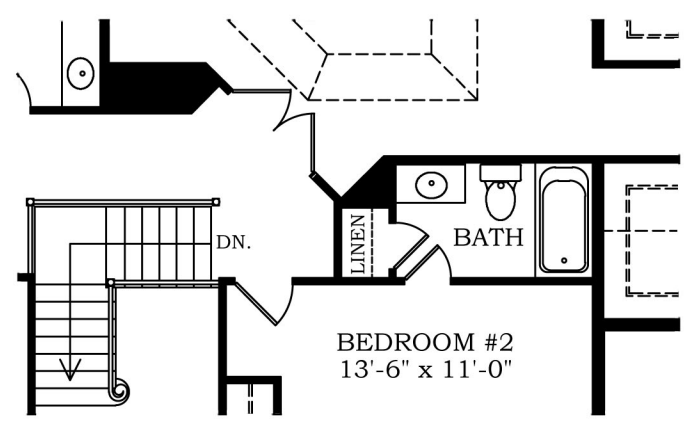
PARTIAL SECOND LEVEL AT OPT. BEDROOM #2 BATH
