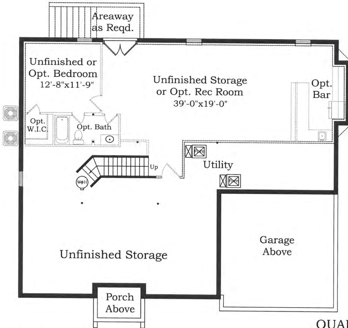
FOUNDATION/ BASEMENT PLAN
